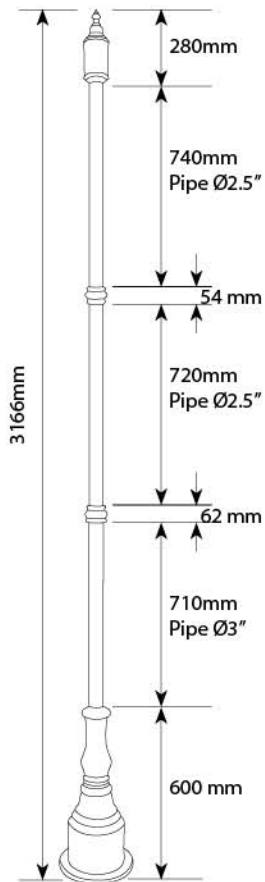
Product Code : P25 Pole Material : Aluminium Casting & Extrusion Base Dia : Ø275 mm
