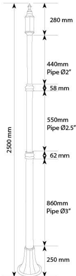
Product Code : P21 Pole Material : Aluminium Casting & Extrusion Base Dia : Ø240 mm
