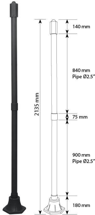
Product Code : P47 Pole Material : Aluminium Casting & Extrusion Base Dia : Ø250 mm
