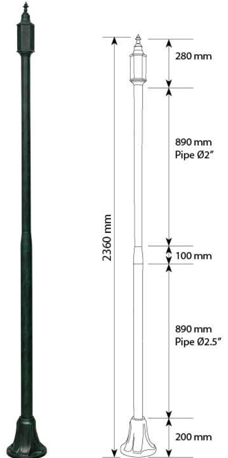
Product Code : P17 Pole Material : Aluminium Casting & Extrusion Base Dia : Ø210 mm
