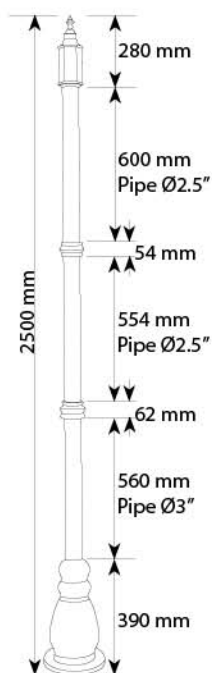
Product Code : P23 Pole Material : Aluminium Casting & Extrusion Base Dia : Ø260 mm
