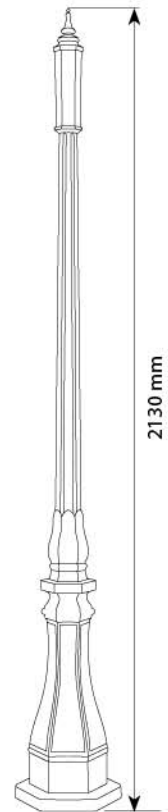
Product Code : P15 Pole Material : Aluminium Die Casting Base Dia : Ø320 mm
