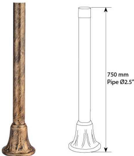
Product Code : P3 Pole Material : Aluminium Casting & Extrusion Base Dia : Ø170 mm
